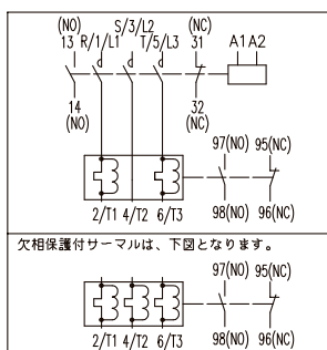
PAK-21JT-SL2C PAK-21JGT-SL2C
