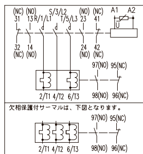
PAK-50HT~150HT-SL2(C) PAK-50HGT~150HGT-SL2(C)
