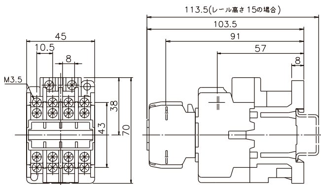
PAK-8JS (8P)
