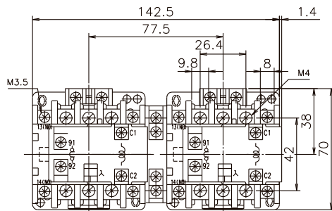
RSK-35JL
