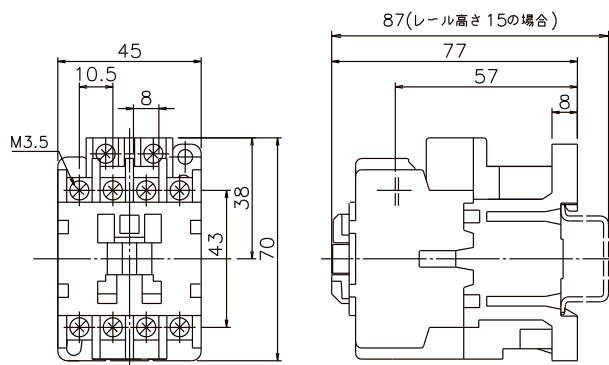
PAK-8JS (4P)
