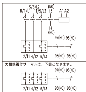
PAK-11JT~20JT-SL2C PAK-11JGT~20JGT-SL2C
